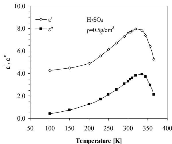
Figure 1. Temperature dependence of dielectric permeability \varepsilon' and dielectric loss \varepsilon'' coefficients (at frequency 1 kHz) for the chemically modified STBF samples by sulphuric acid.
