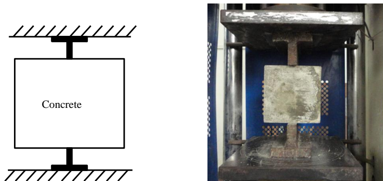
(b). Test schematic for splitting tensile strength
