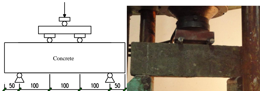
(c). Test schematic for flexural strength
