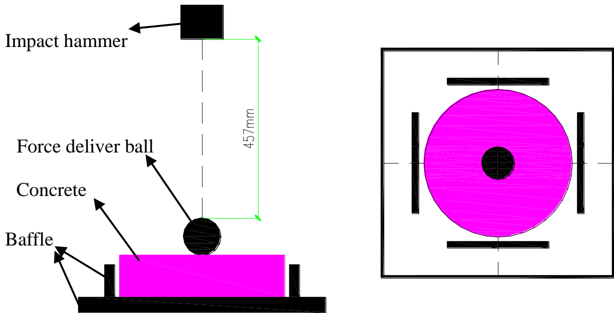
Fig. (2). Equipment for impact behavior test.
