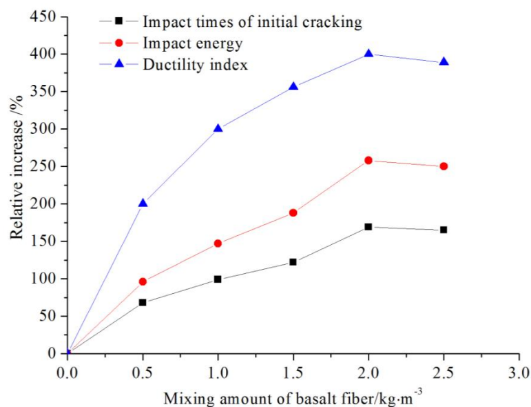
Fig. (6). Relationship between the mixing amount of basalt fiber and the impact toughness.
