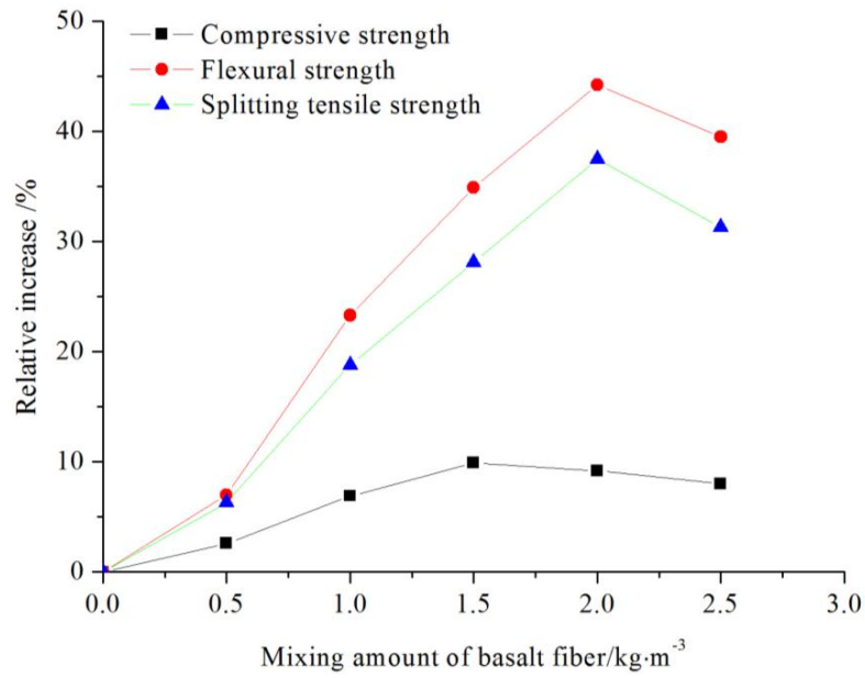
Fig. (3). Relationship between the mixing amount of basalt fiber and the mechanical characteristics.
